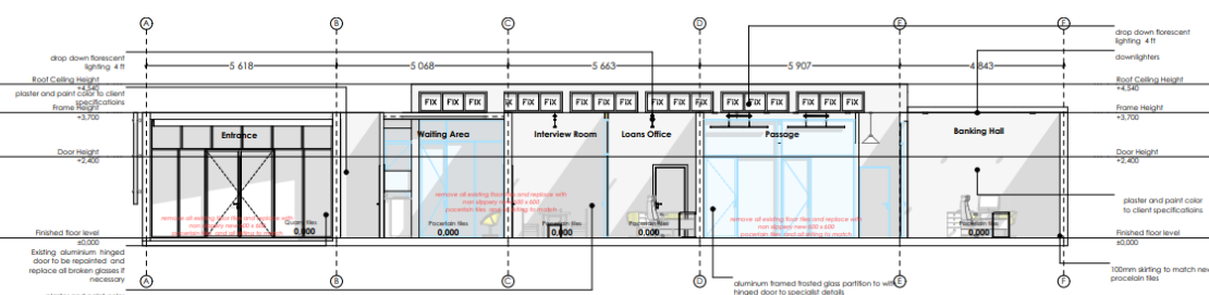
Section I-I Scale 1:50
