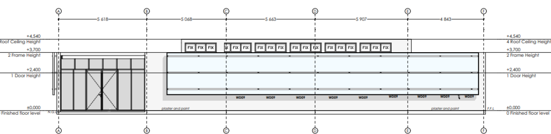
FRONT ENTRANCE Scale 1:50
