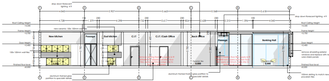
Section H-H Scale 1:50
