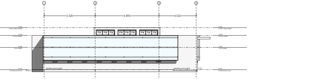
SIDE ELEVATION Scale 1:50
